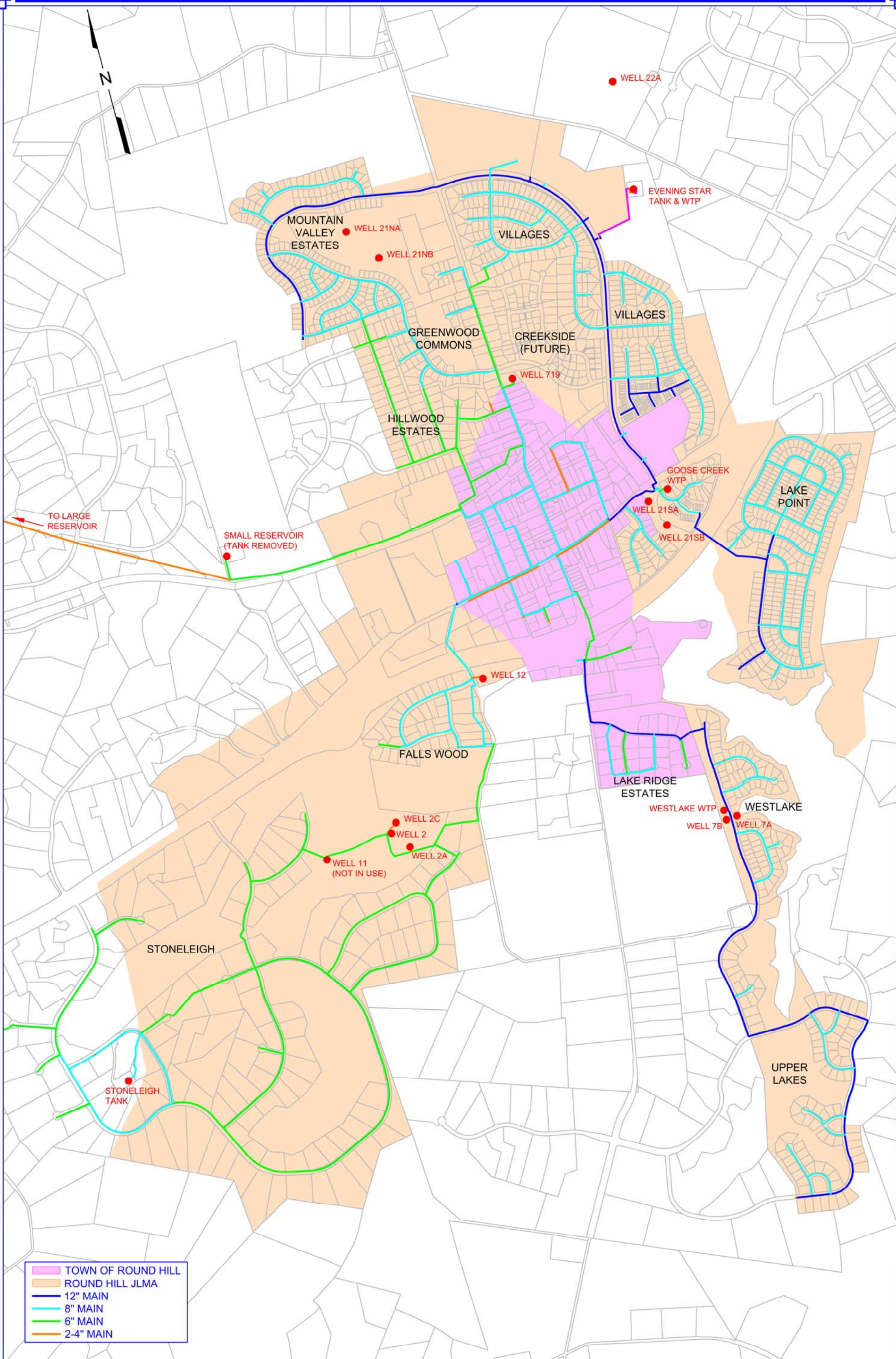
FIGURE A: Round Hill Water System Service Area Map
